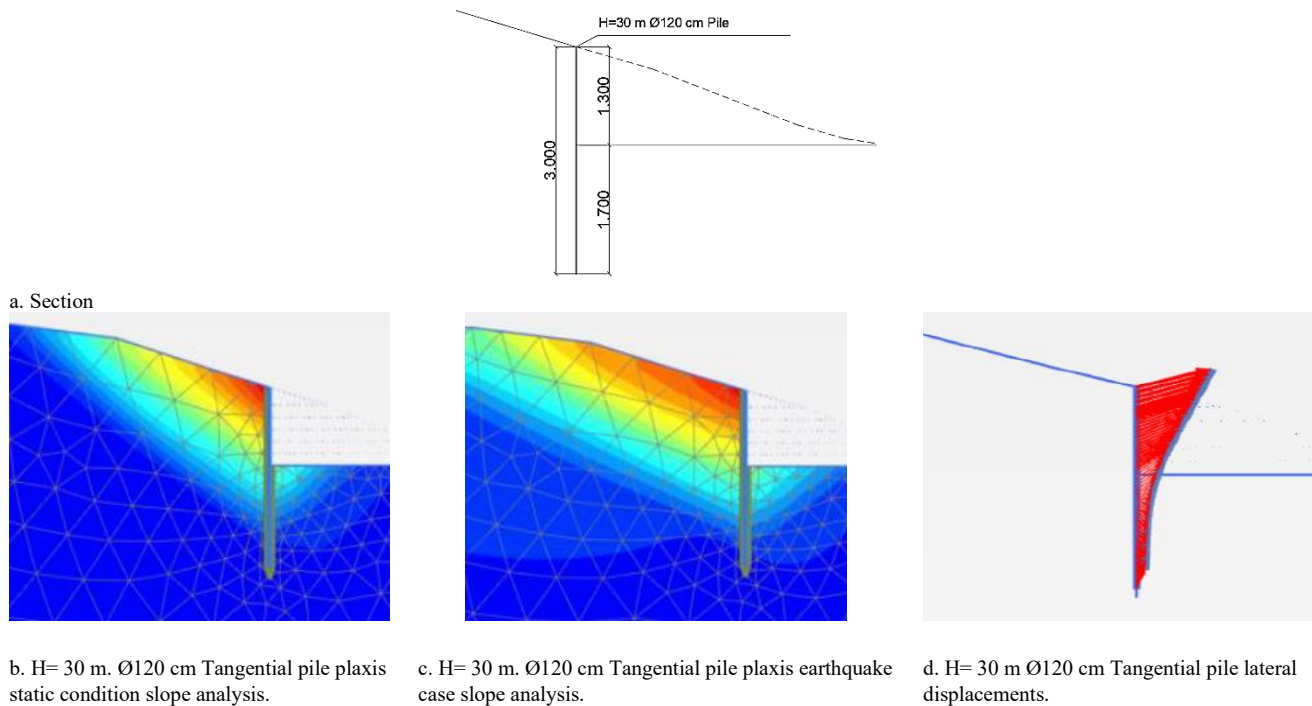
Figure 16. H=30.00 m Ø 120 cm tangent pile dimensions and slope analysis results.
