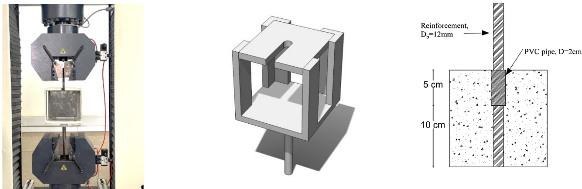
Fig. 3. Test setup and specimen for direct pull out test.
