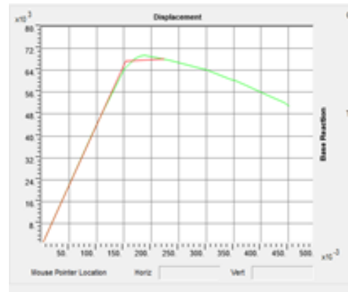
Fig 4. Capacity curve FEMA-356
