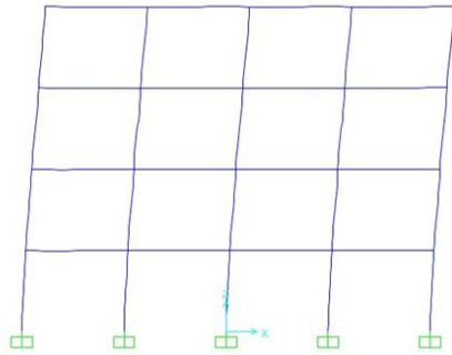
Fig5. Deformed shape of the frame at Step1
