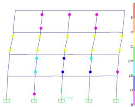
Fig9. Deformed shape of the frame at Step8
