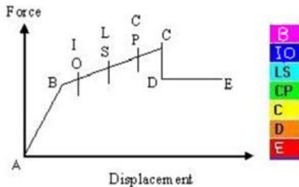
Fig.1 Different stages of plastic hinge
