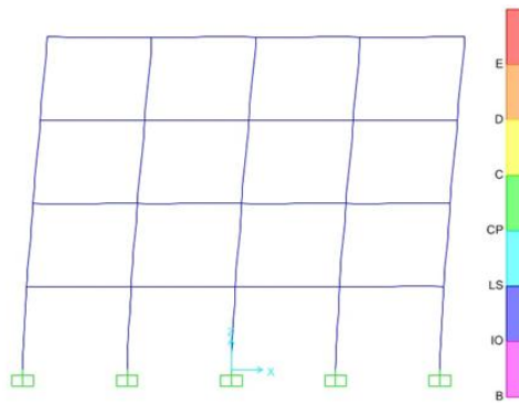
Fig6. Deformed shape of the frame at Step3
