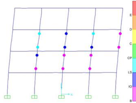
Fig7. Deformed shape of the frame at Step4
